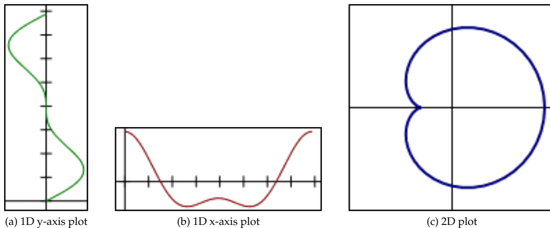
Figure 7: FunctionPlot
