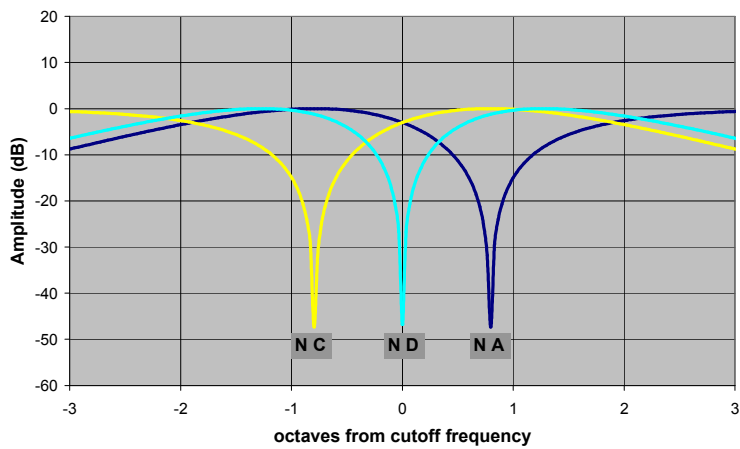
Notch Frequency Responses -- Zero Resonance
