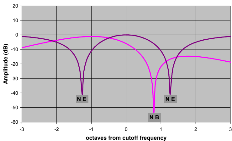
Notch Frequency Responses -- Zero Resonance
