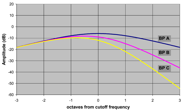
Band Pass Frequency Responses -- Zero Resonance
